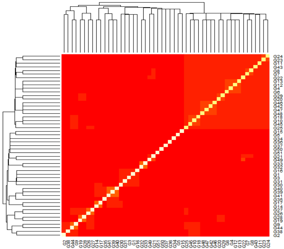
Supplementary Figure 3: The dendrograms of 51 genotypes generated by pedigree based analysis of the relationship matrix. Heatmap of the additive relationship matrix shows family structure. Individuals derived from the same full-sib family share a common symbol.
